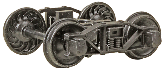
50-Ton Freight Truck
