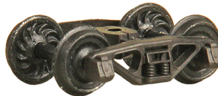
#722 A.S.F.® A-3 Ride-Control® Truck
