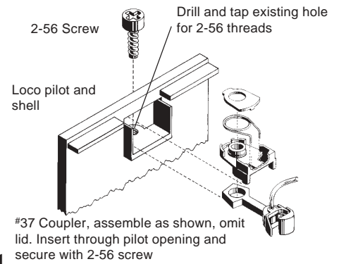
Fig.1 #37 Installation
