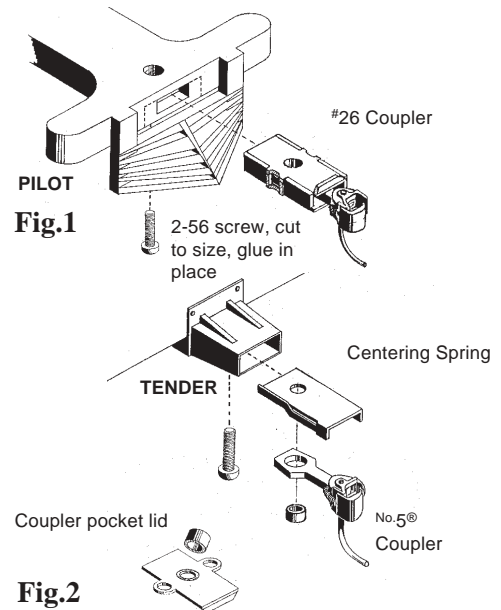
#26 Pilot, No.5® Tender Installation
