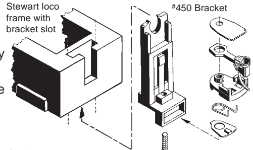
Fig.1 Screw, included with #450 #450 Installation 30-Series Draft Gear Box with No. 5® Coupler, included with the #450 Coupler Conversion package
