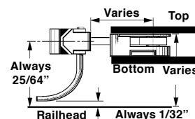
Centering Spring
